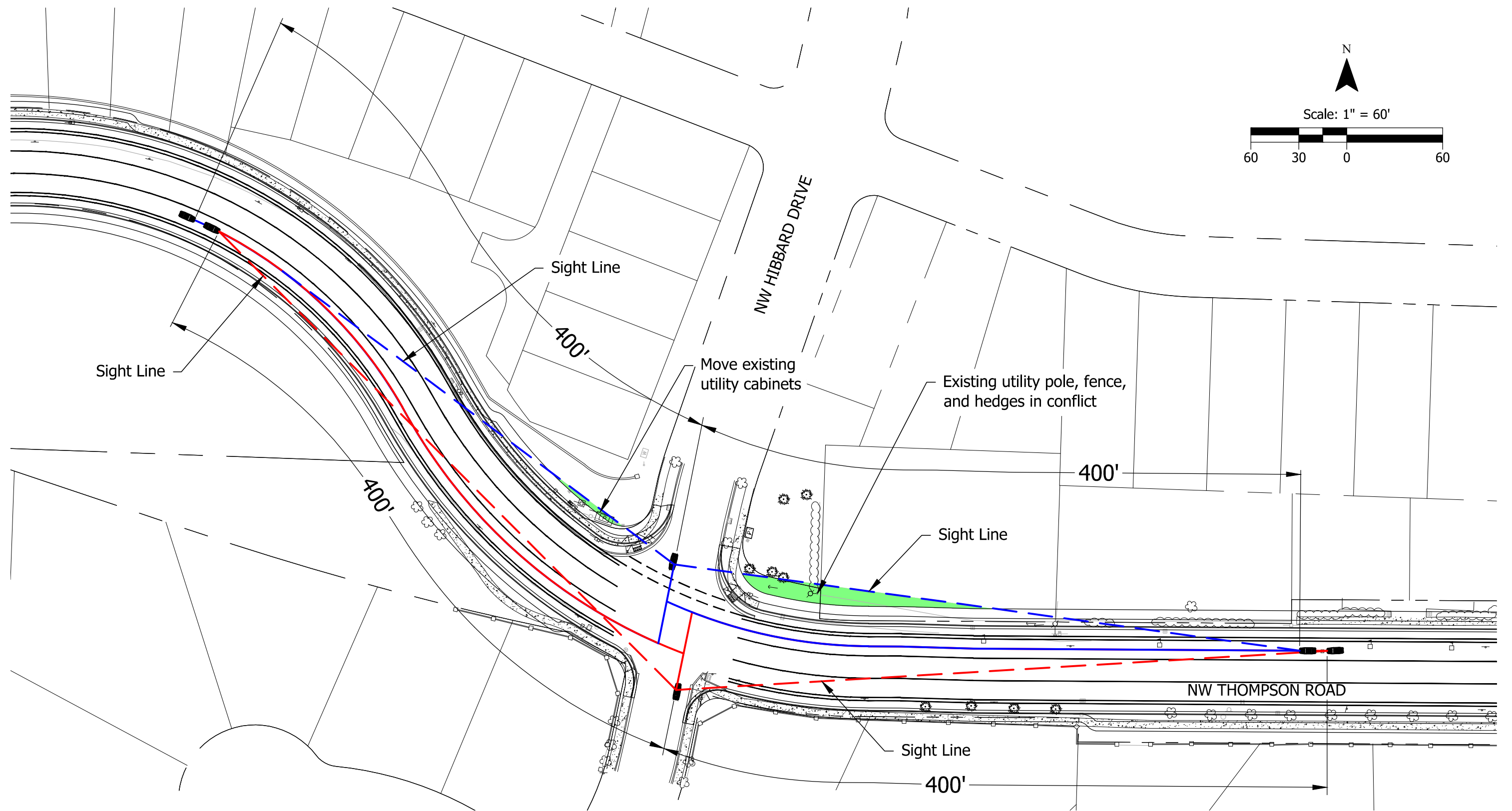
Intersection Sight Distance (Proposed - 15' Offset) Washington County, OR
